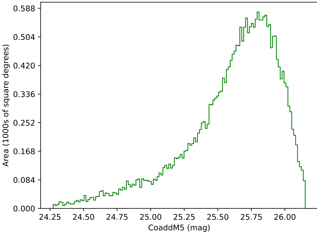
start_date_do-360v3.4_10yrs Yr 1 g band: CoaddM5
