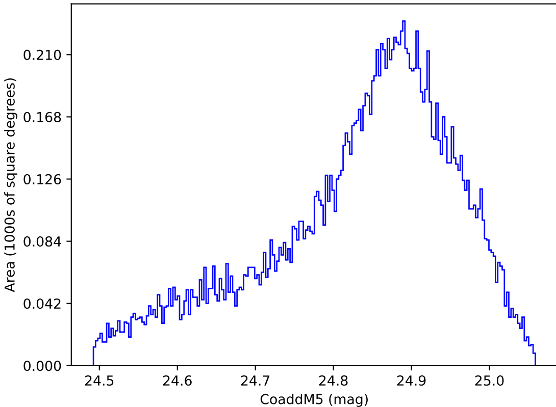
start_date_do-360v3.4_10yrs WFD y band: CoaddM5
