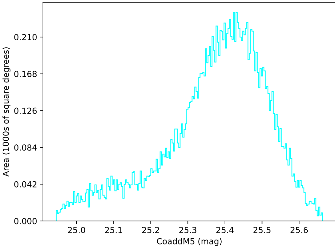
start_date_do-360v3.4_10yrs WFD u band: CoaddM5
