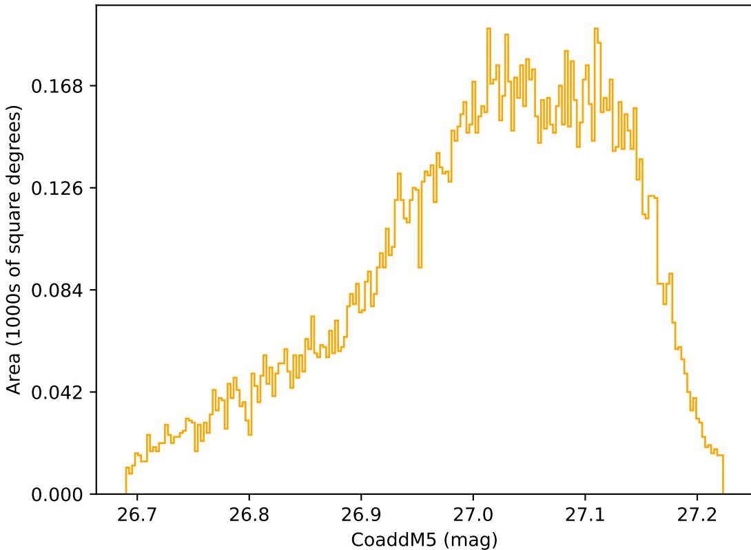
start_date_do-360v3.4_10yrs WFD r band: CoaddM5
