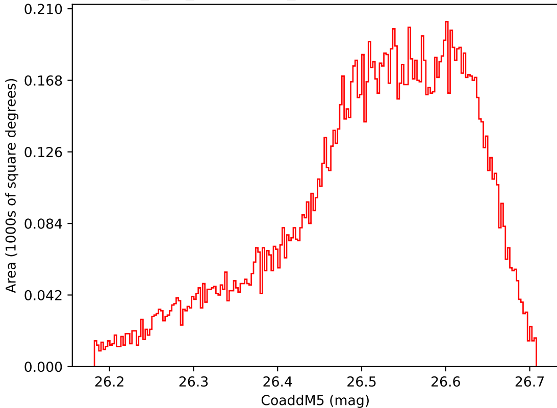
start_date_do-360v3.4_10yrs WFD i band: CoaddM5
