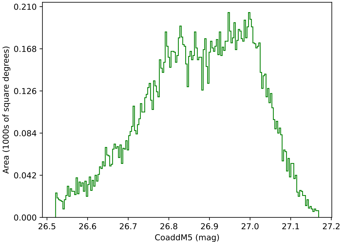
start_date_do-360v3.4_10yrs WFD g band: CoaddM5
