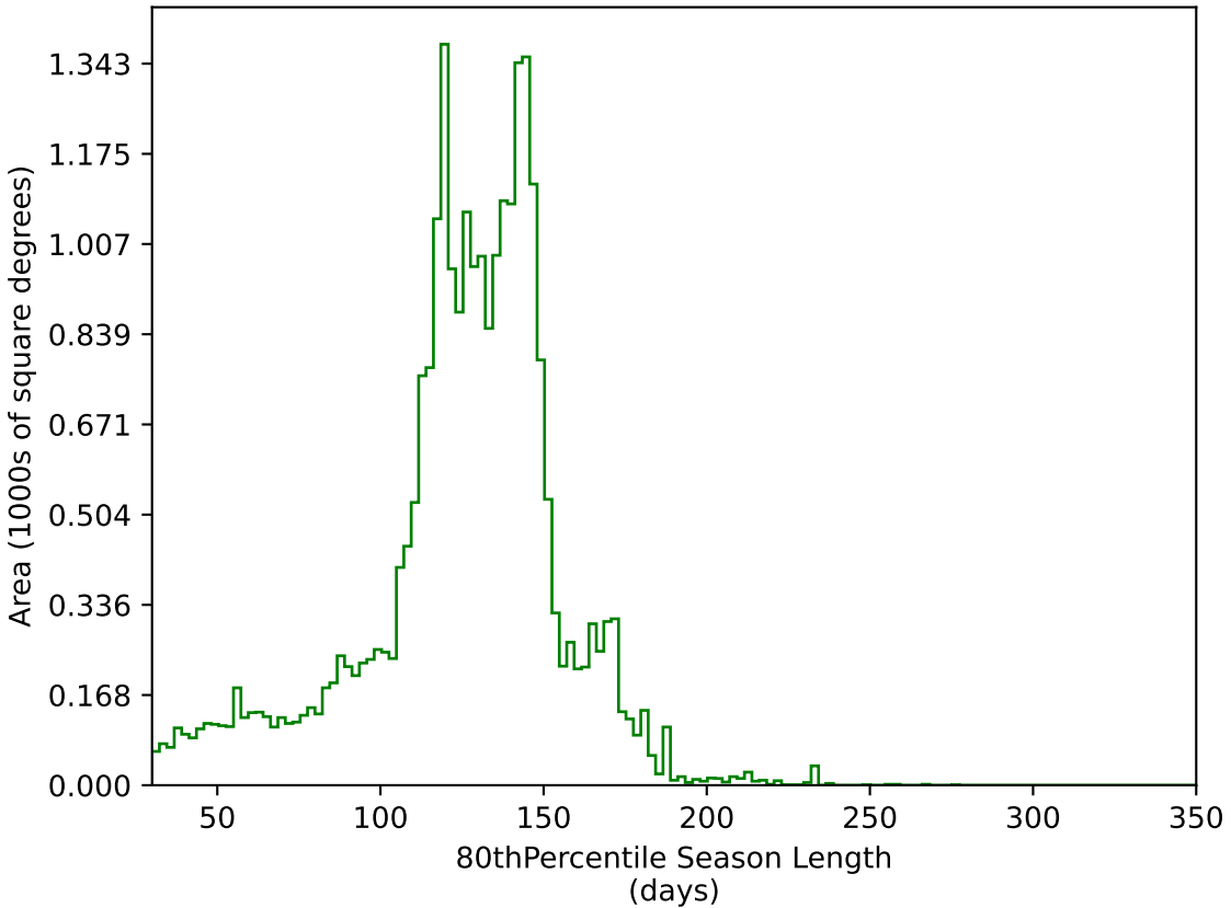
start_date_do-360v3.4_10yrs All sky g band: 80thPercentile Season Length
