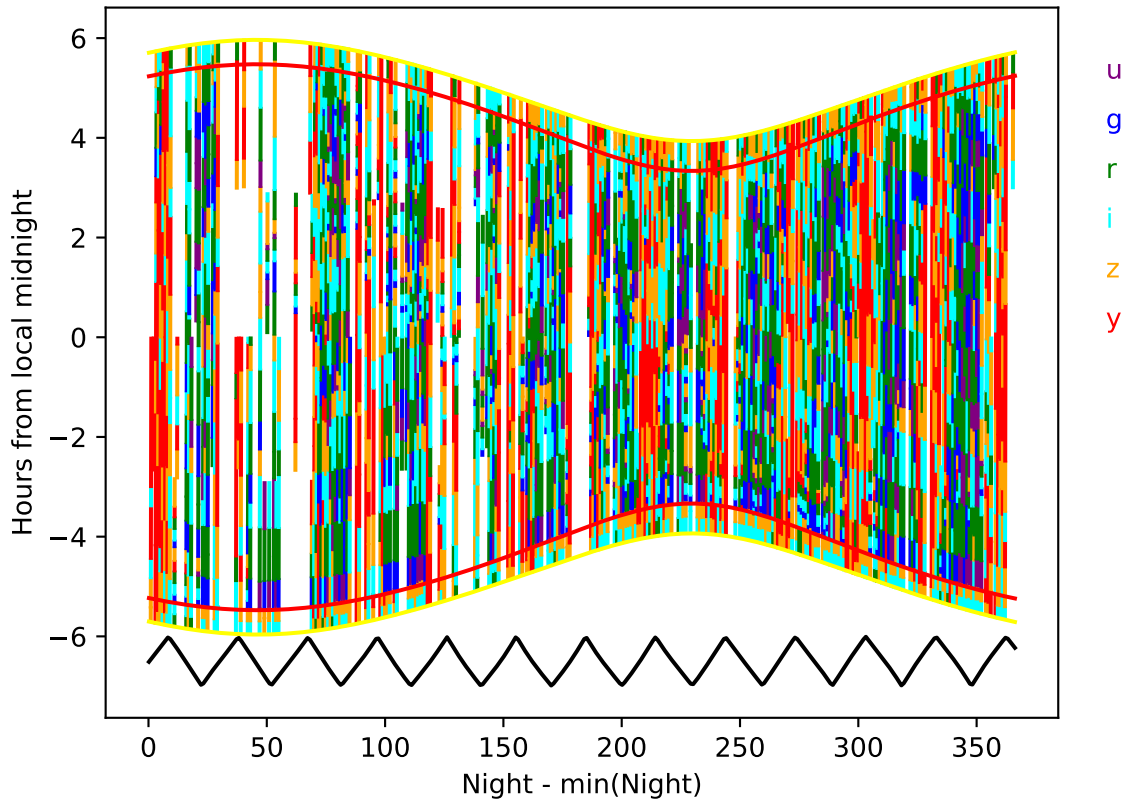
start_date_do-360v3.4_10yrs year 9-10: Hourglass
