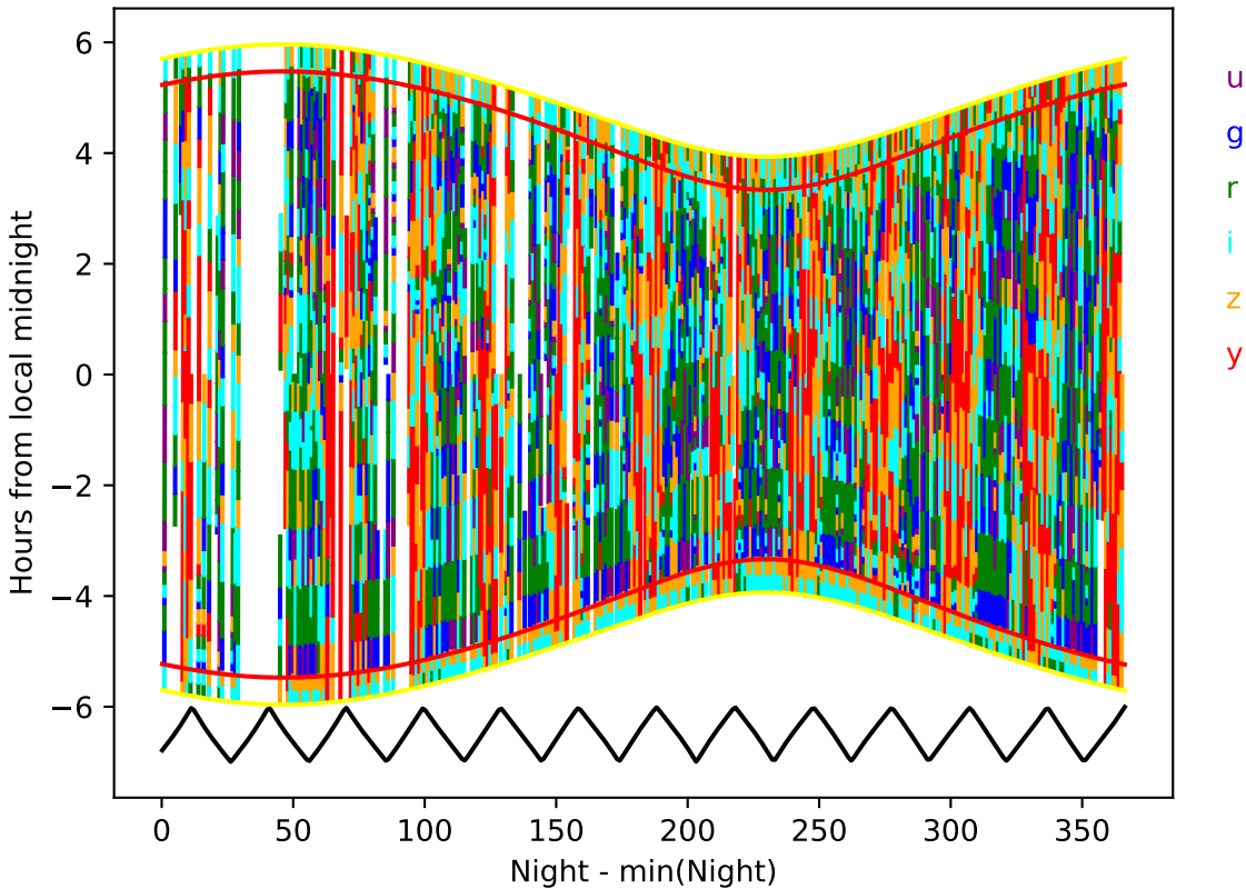
start_date_do-360v3.4_10yrs year 6-7: Hourglass
