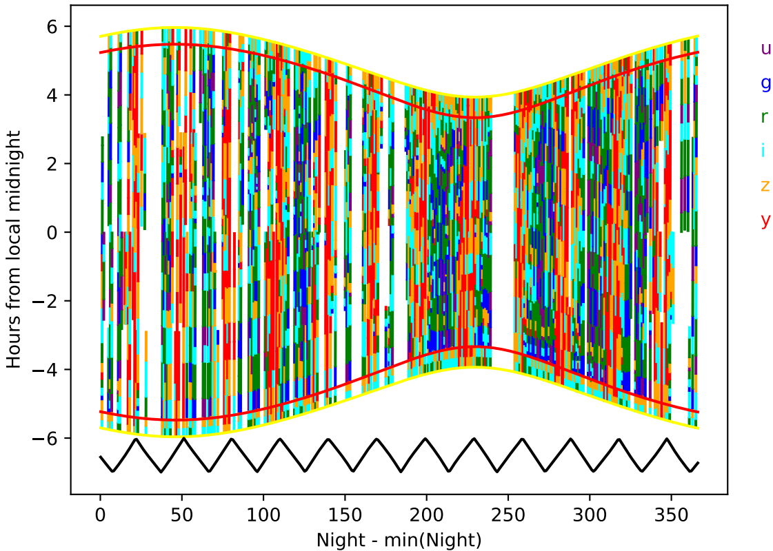
start_date_do-360v3.4_10yrs year 5-6: Hourglass
