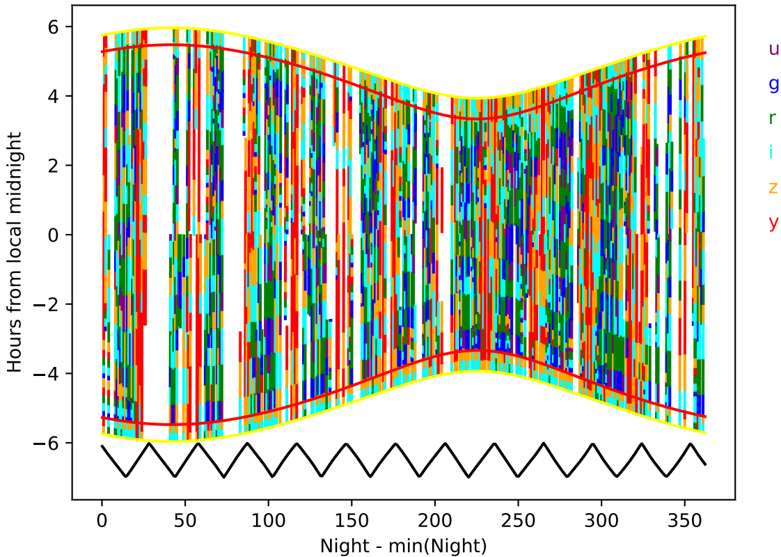
start_date_do-360v3.4_10yrs year 4-5: Hourglass
