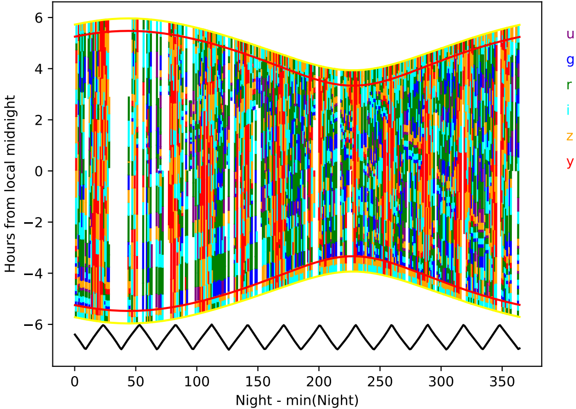
start_date_do-360v3.4_10yrs year 2-3: Hourglass
