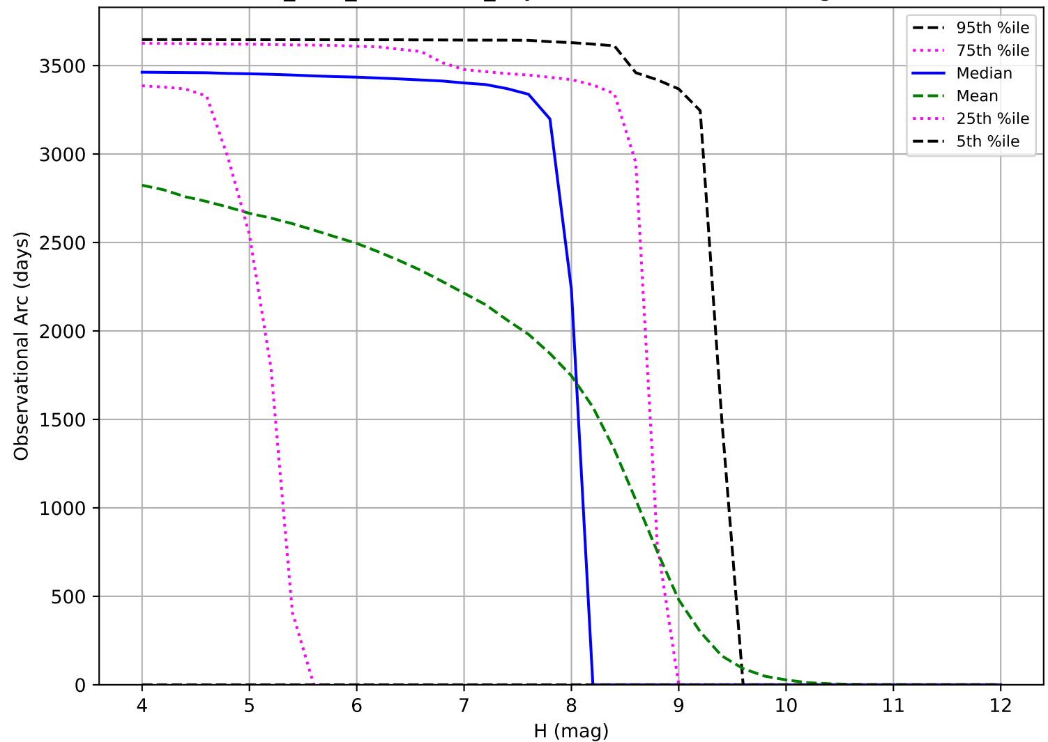
start_date_do-270v3.4_10yrs: Observational Arc Length TNO
