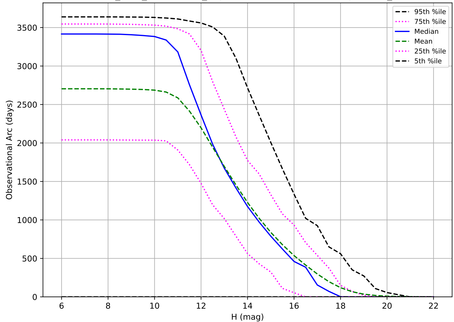
start_date_do-270v3.4_10yrs: Observational Arc Length OCC_r5
