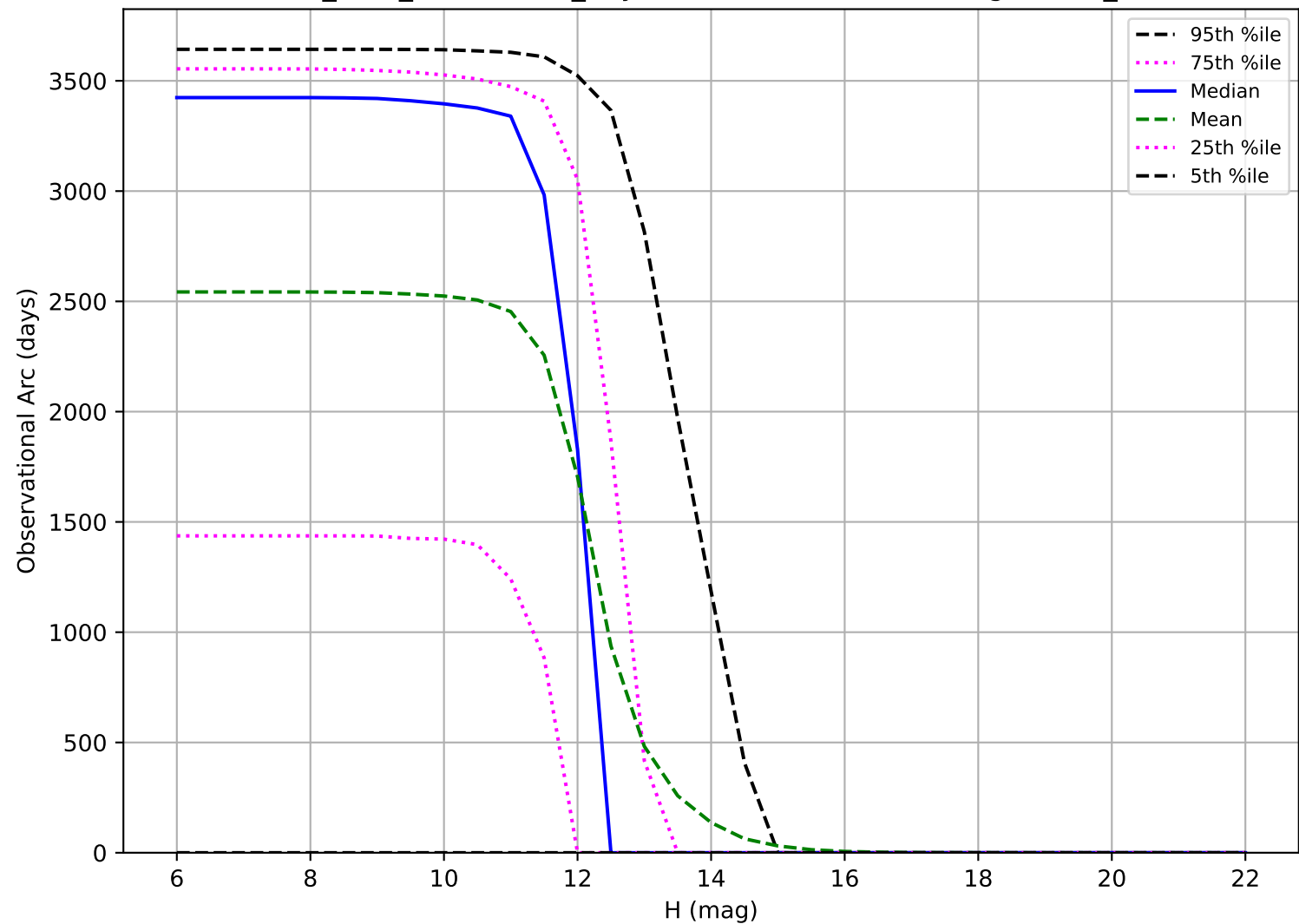
start_date_do-270v3.4_10yrs: Observational Arc Length OCC_r20
