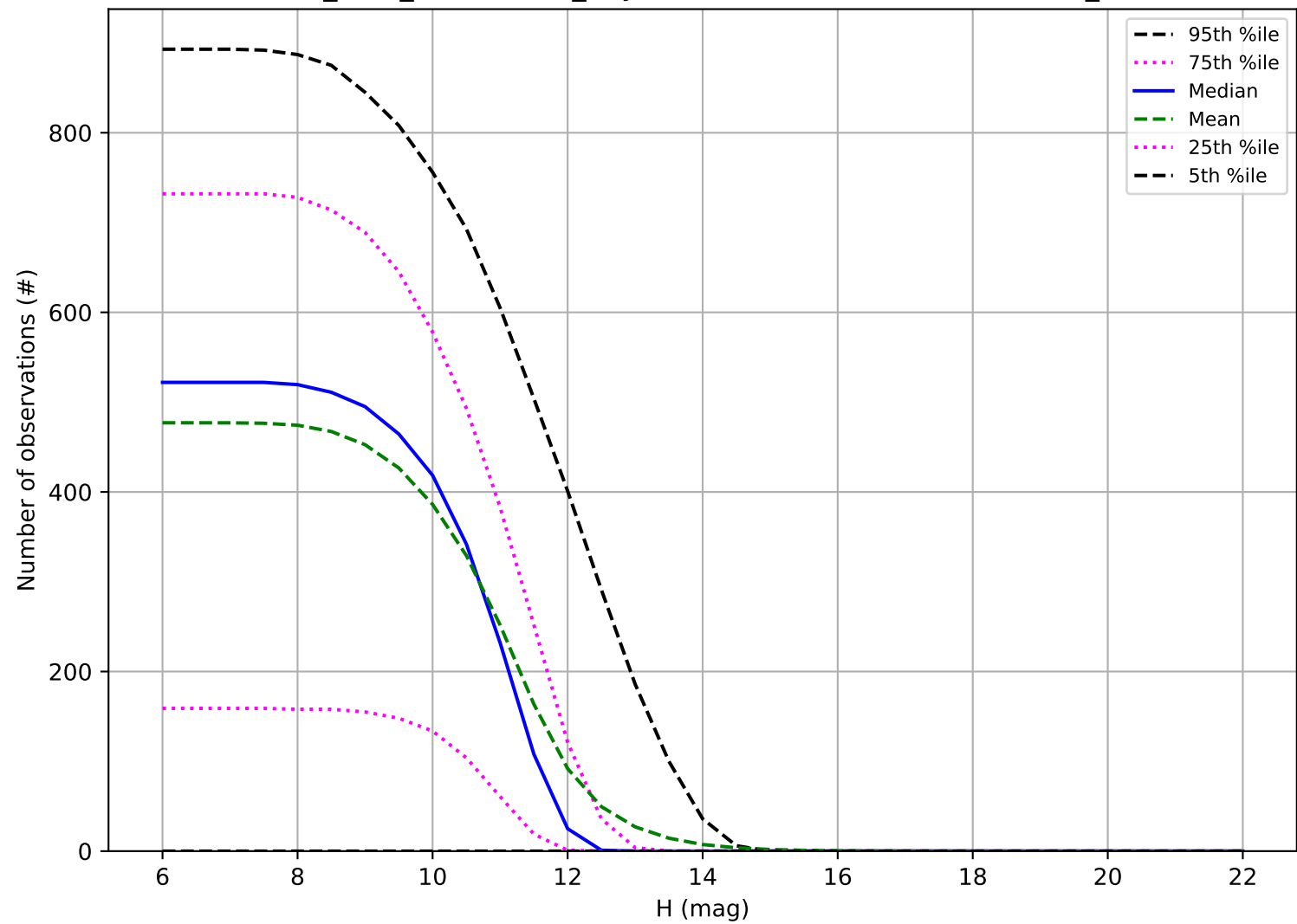
start_date_do-270v3.4_10yrs: Number of observations OCC_r20
