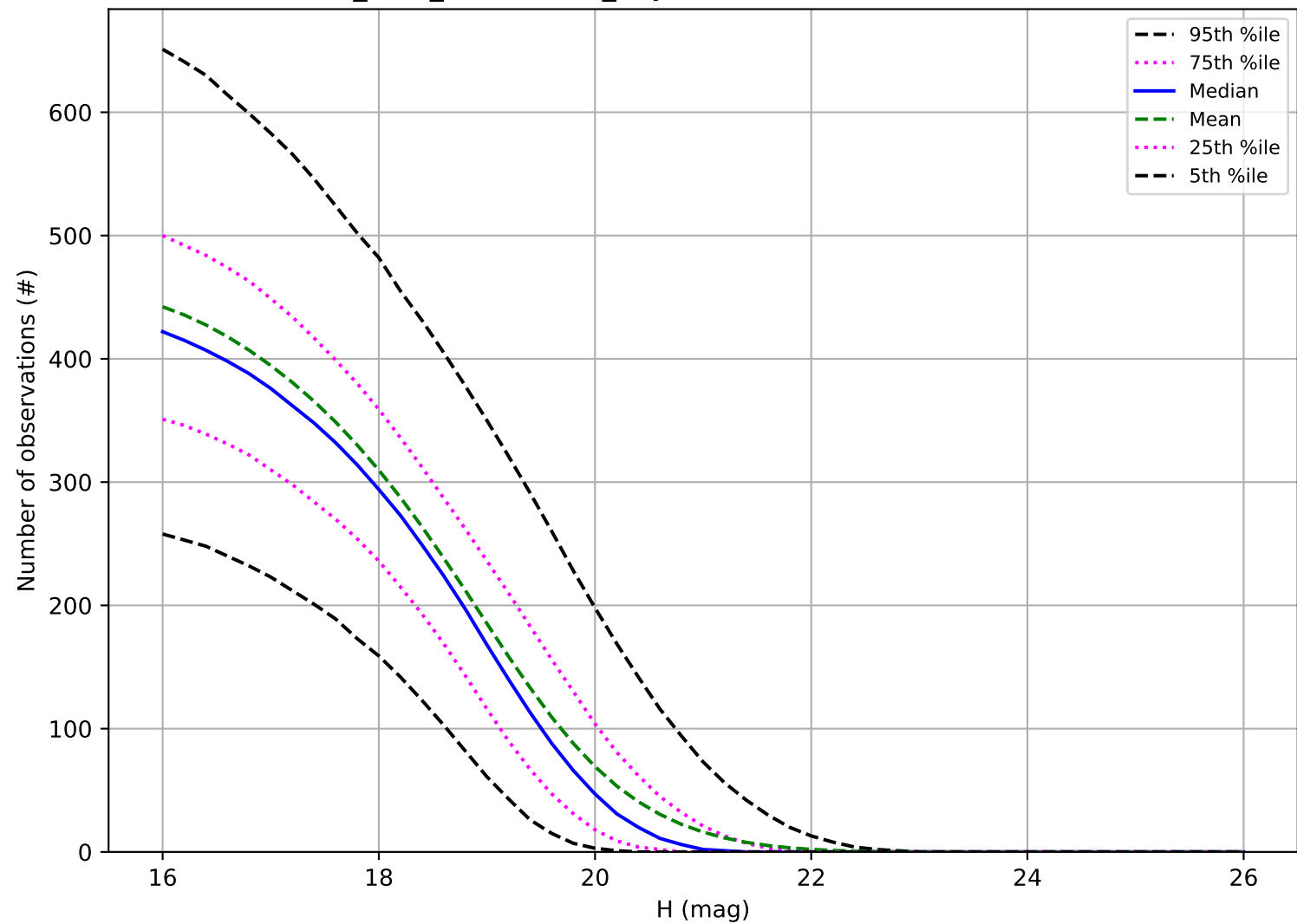
start_date_do-270v3.4_10yrs: Number of observations MBA
