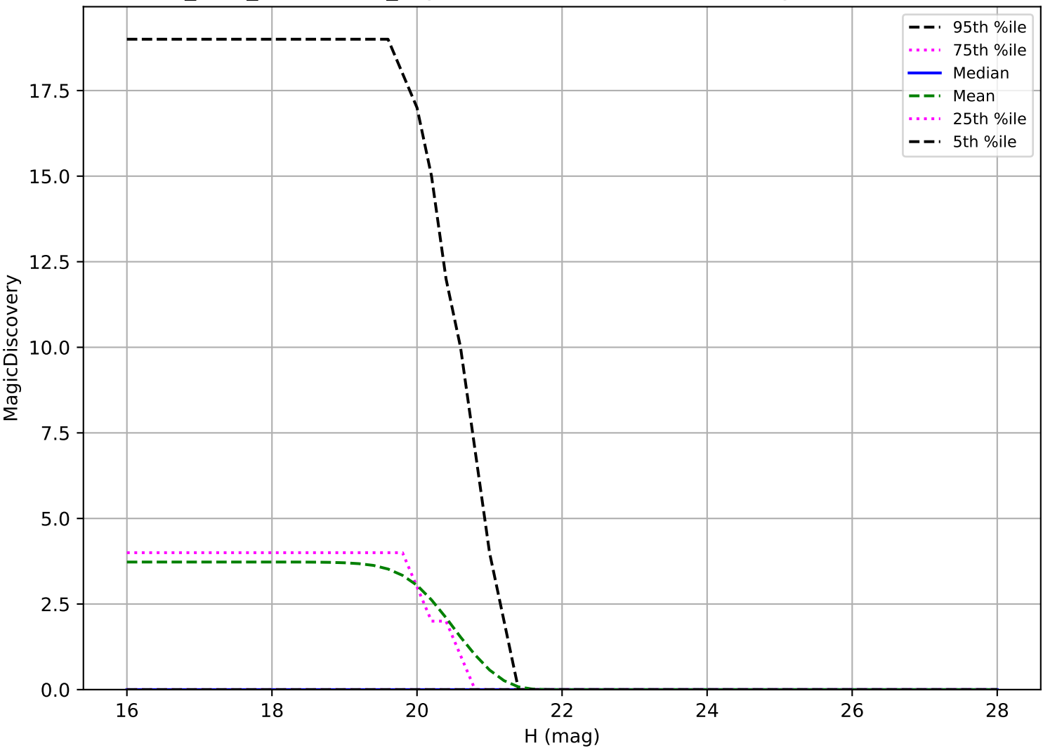
start_date_do-270v3.4_10yrs: Vatira 6 detections in 60 nights detection loss
