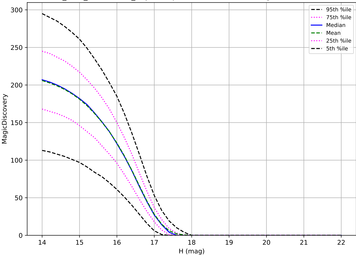
start_date_do-270v3.4_10yrs: Trojan 6 detections in 60 nights detection loss
