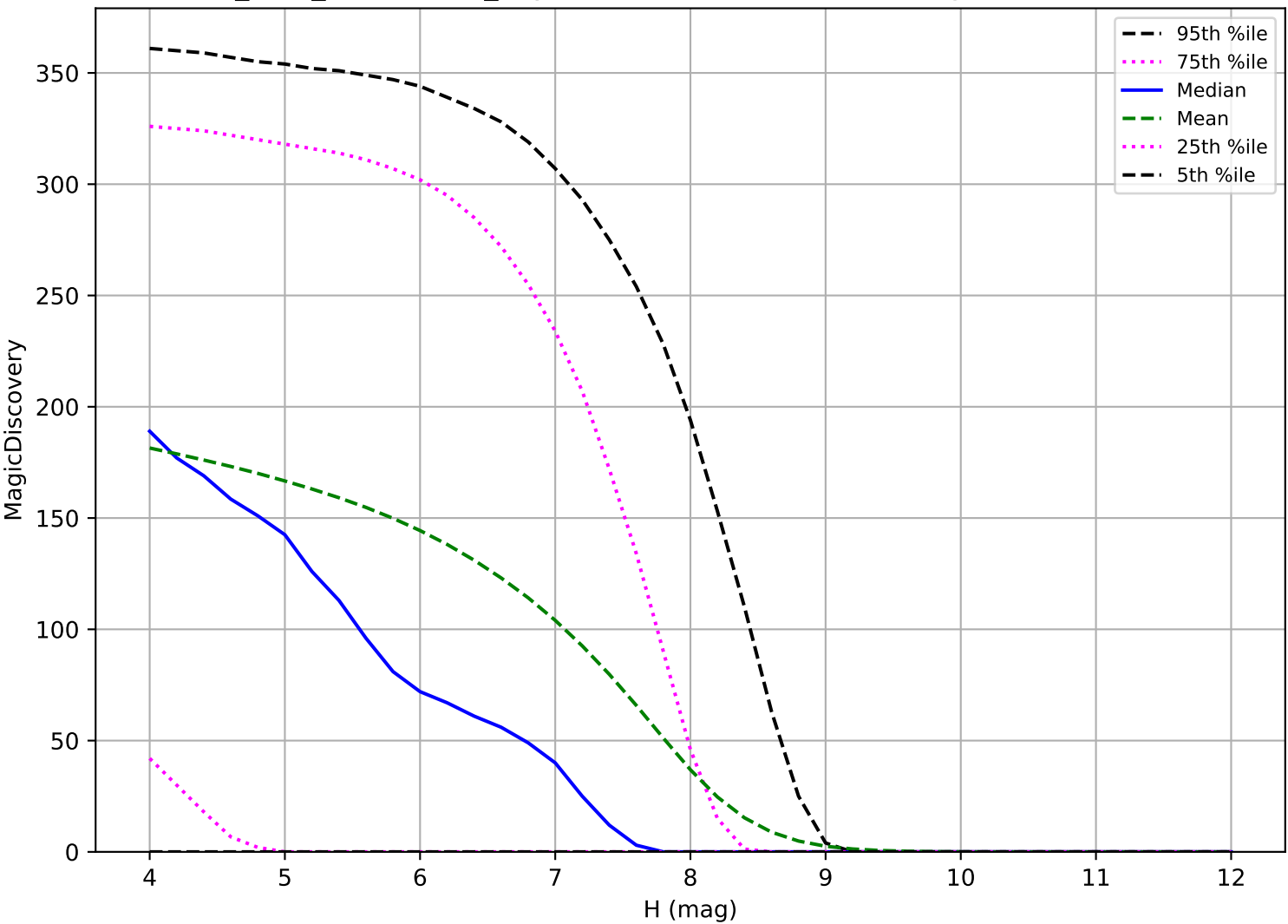
start_date_do-270v3.4_10yrs: TNO 6 detections in 60 nights detection loss
