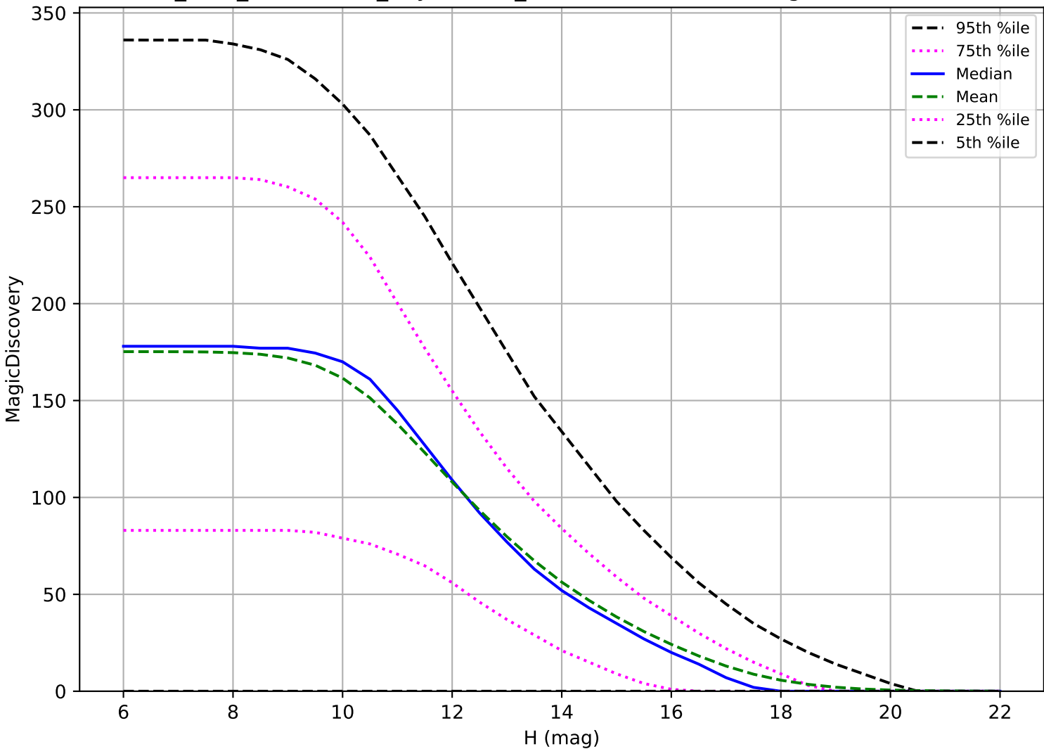
start_date_do-270v3.4_10yrs: OCC_r5 6 detections in 60 nights detection loss
