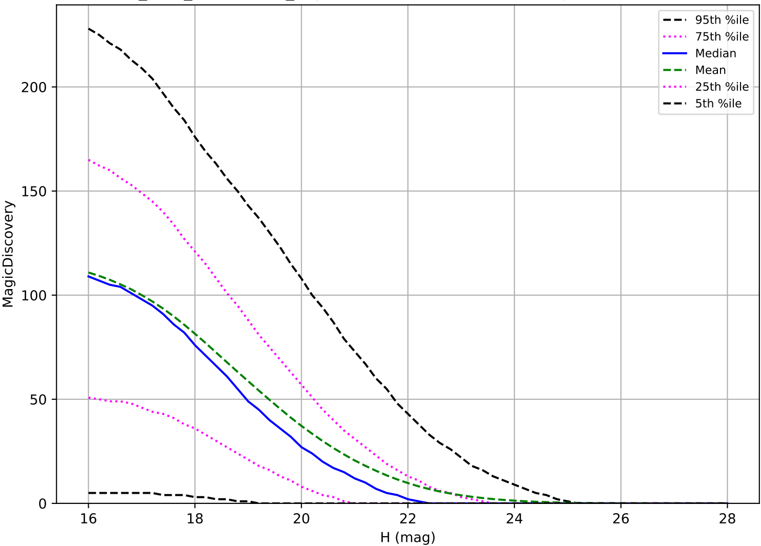
start_date_do-270v3.4_10yrs: NEO 6 detections in 60 nights detection loss
