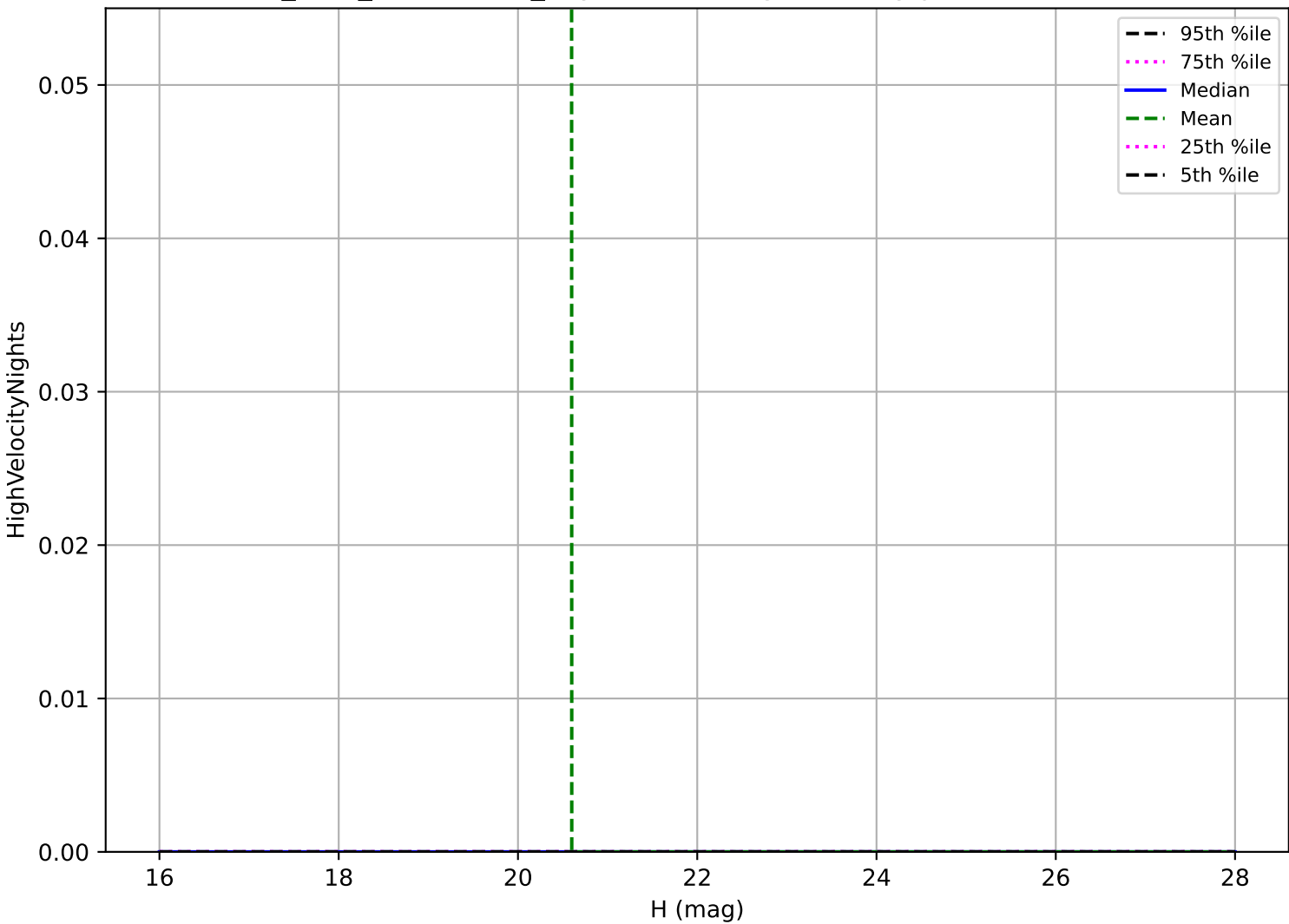
start_date_do-270v3.4_10yrs: Vatira High velocity pair detection loss
