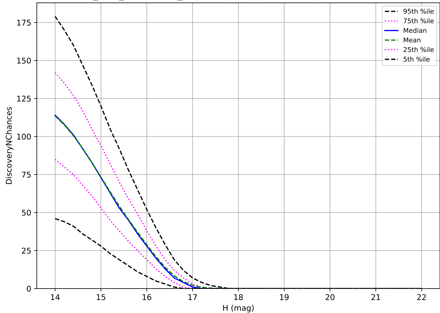
start_date_do-270v3.4_10yrs: Trojan 3 pairs in 15 nights detection loss
