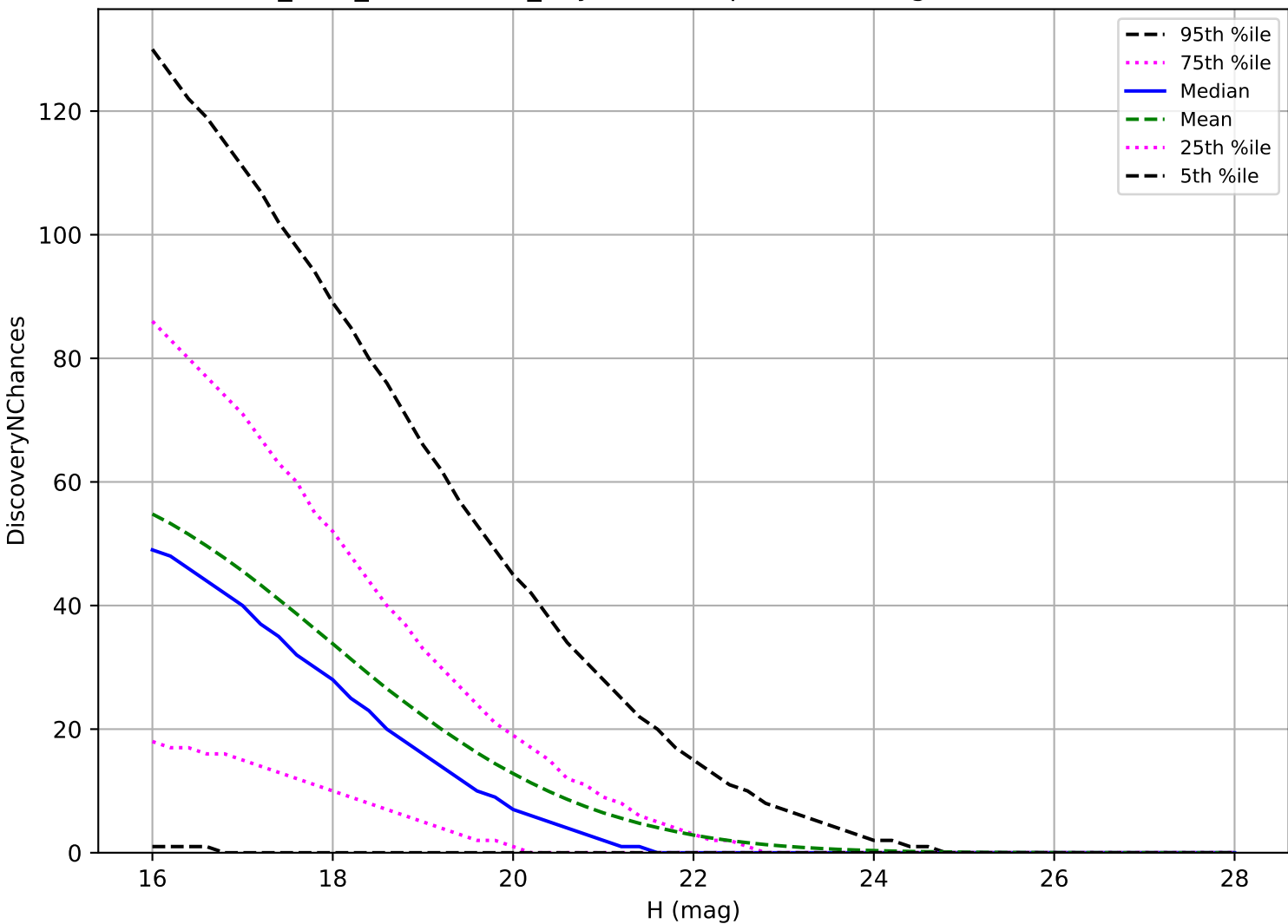
start_date_do-270v3.4_10yrs: PHA 3 pairs in 15 nights detection loss
