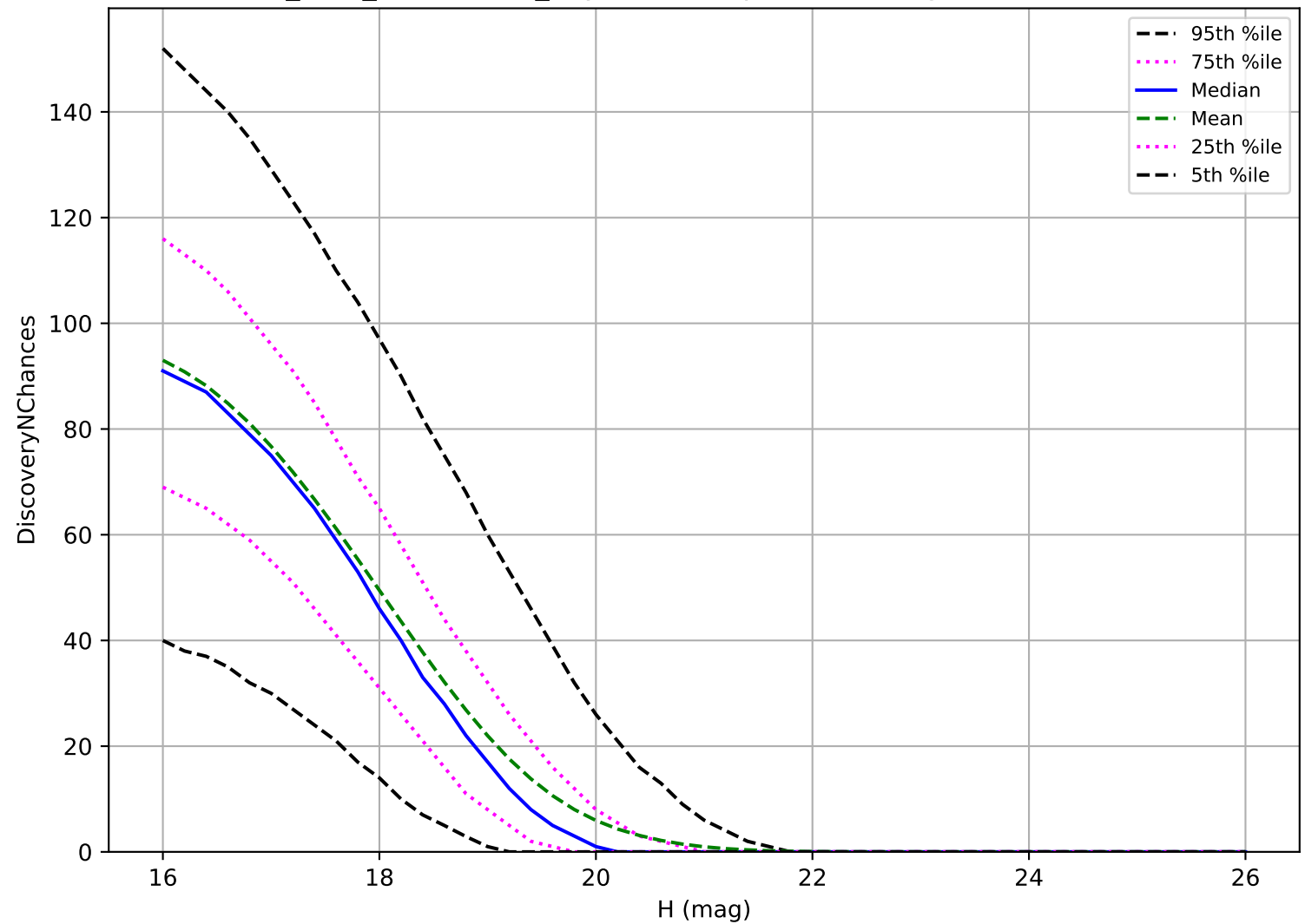
start_date_do-270v3.4_10yrs: MBA 3 pairs in 15 nights detection loss
