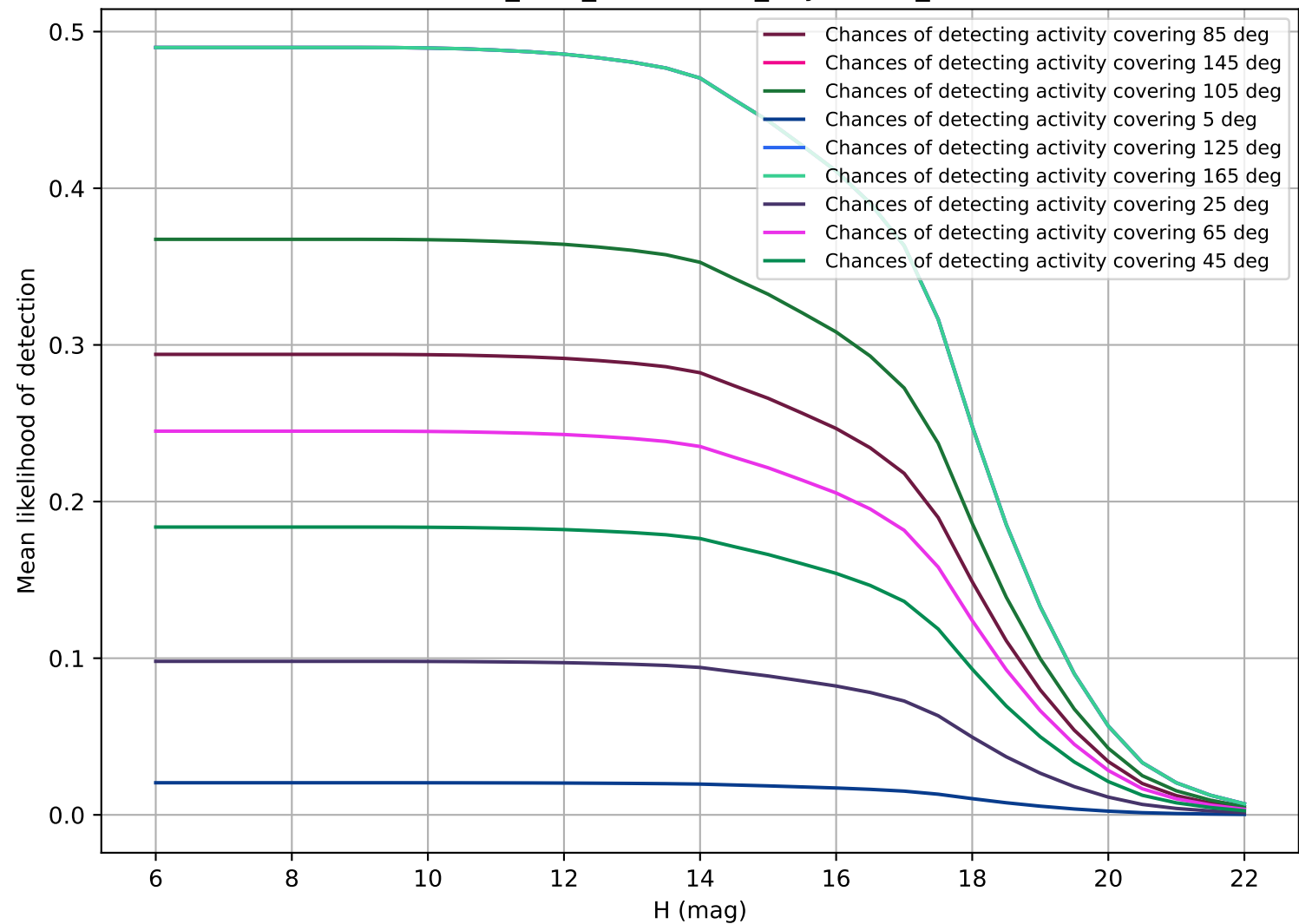
start_date_do-270v3.4_10yrs OCC_r5
