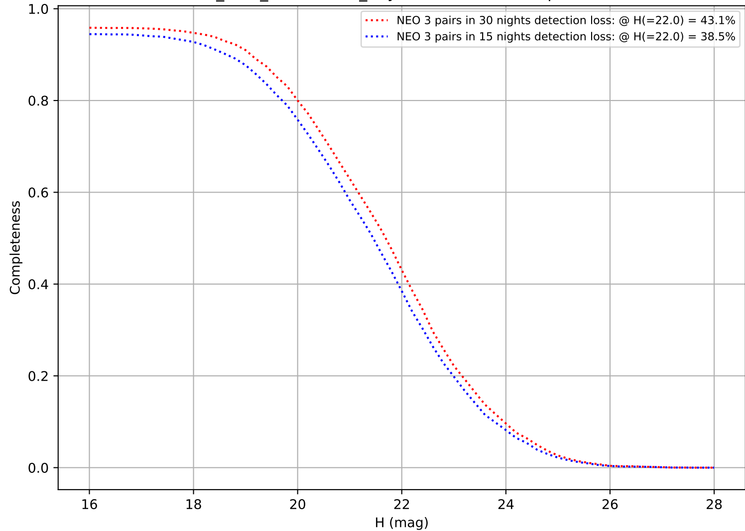
start_date_do-270v3.4_10yrs: DifferentialCompleteness
