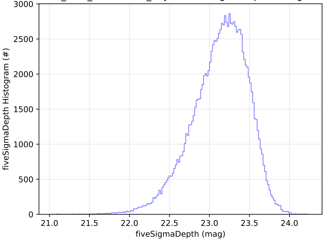
start_date_do-270v3.4_10yrs u: fiveSigmaDepth Histogram
