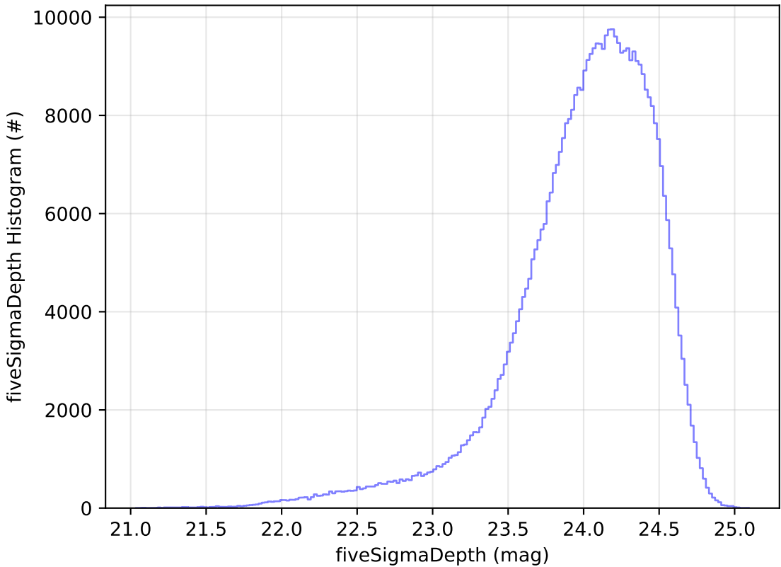
start_date_do-270v3.4_10yrs r: fiveSigmaDepth Histogram
