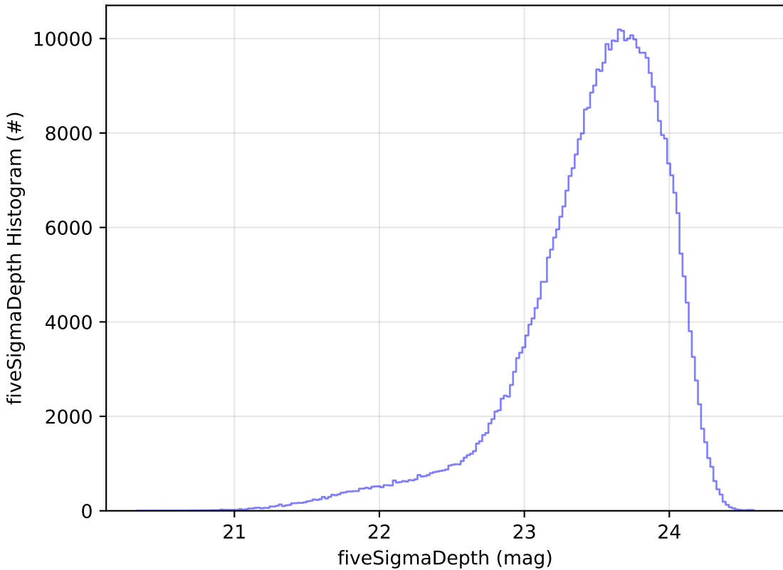
start_date_do-270v3.4_10yrs i: fiveSigmaDepth Histogram
