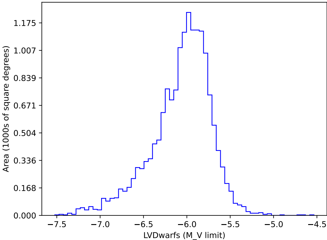
start_date_do-270v3.4_10yrs gi: LVDwarfs
