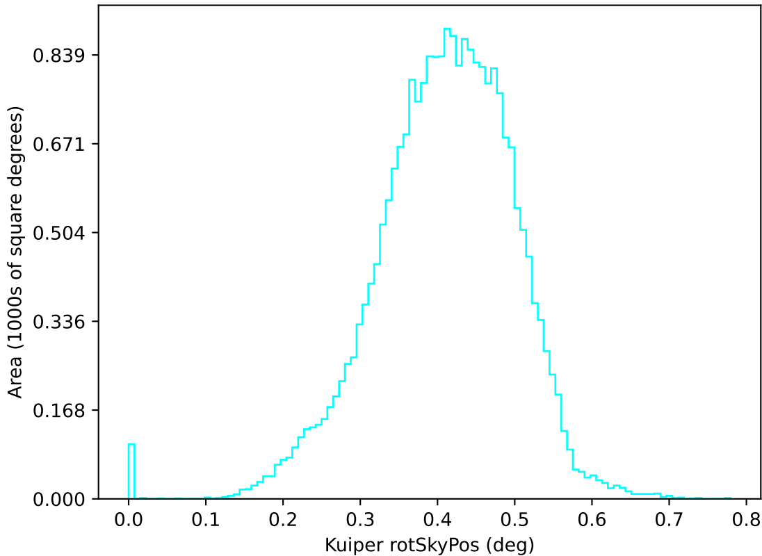
start_date_do-270v3.4_10yrs u: Kuiper rotSkyPos
