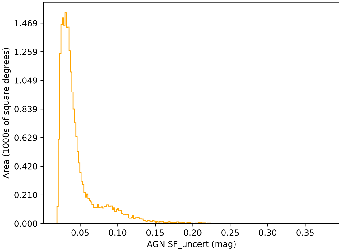
start_date_do-270v3.4_10yrs r band: AGN SF_uncert
