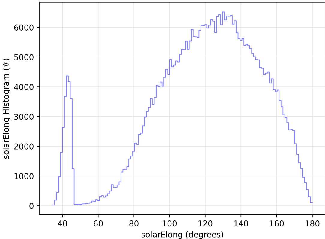
start_date_do-270v3.4_10yrs WFD z band: solarElong Histogram
