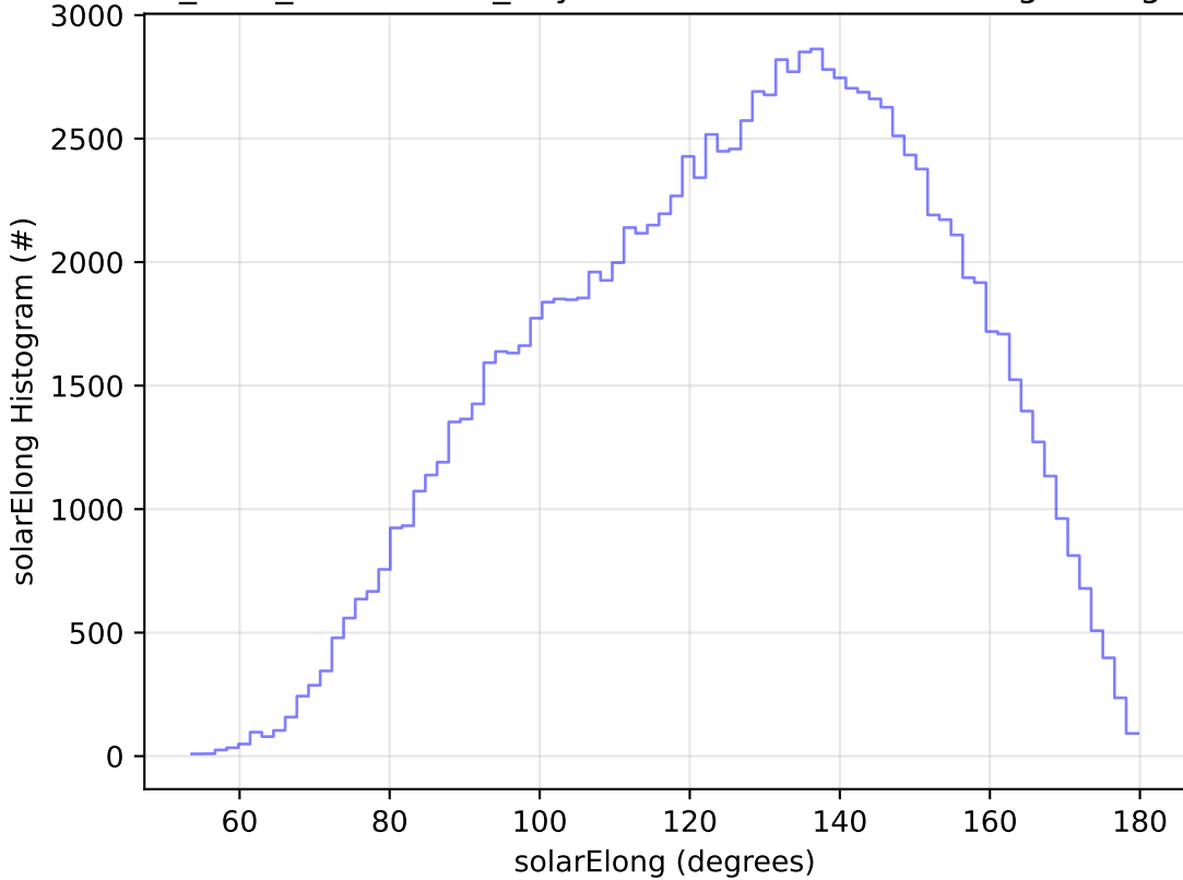
start_date_do-270v3.4_10yrs WFD u band: solarElong Histogram
