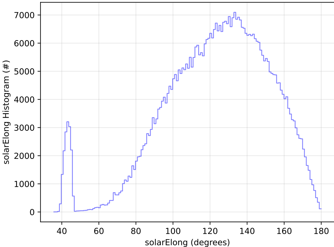
start_date_do-270v3.4_10yrs WFD r band: solarElong Histogram
