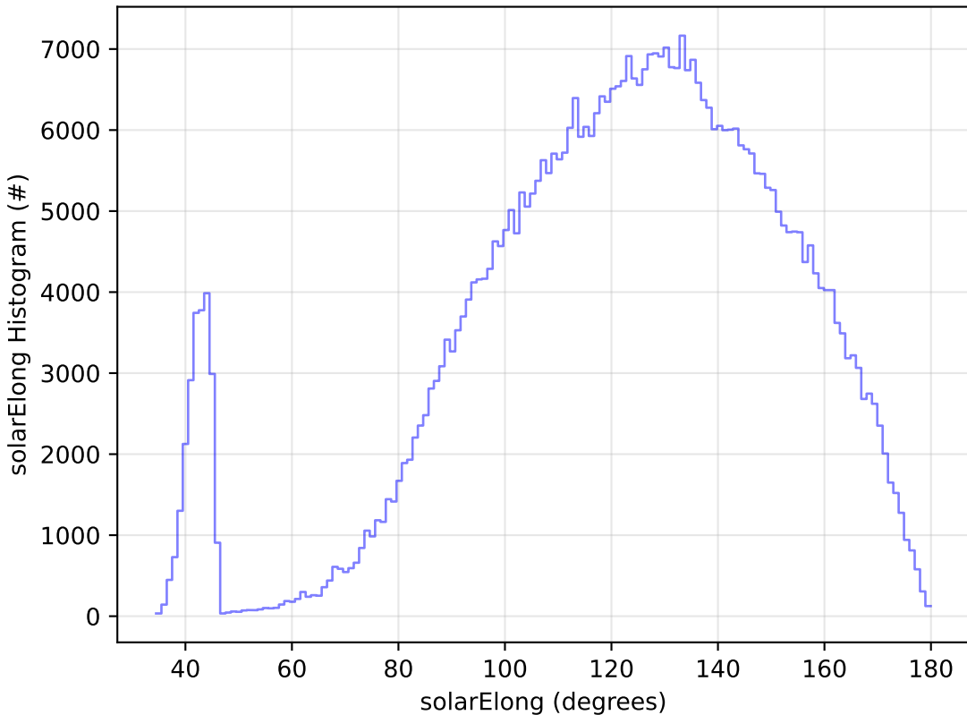
start_date_do-270v3.4_10yrs WFD i band: solarElong Histogram
