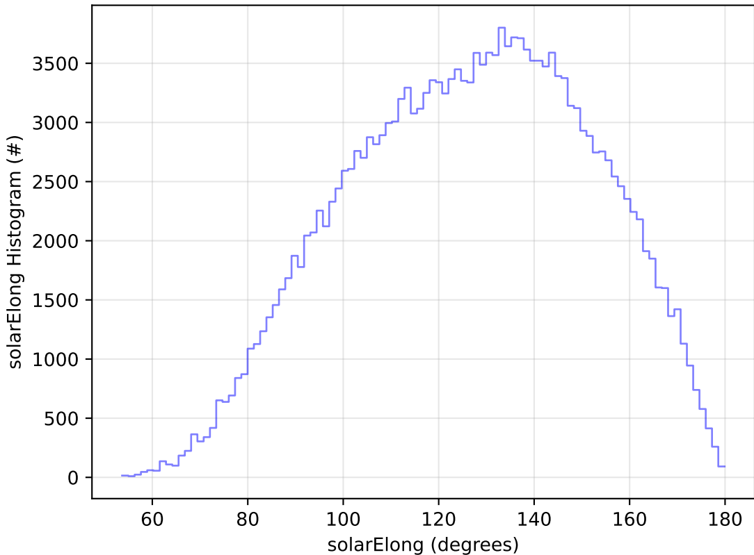
start_date_do-270v3.4_10yrs WFD g band: solarElong Histogram
