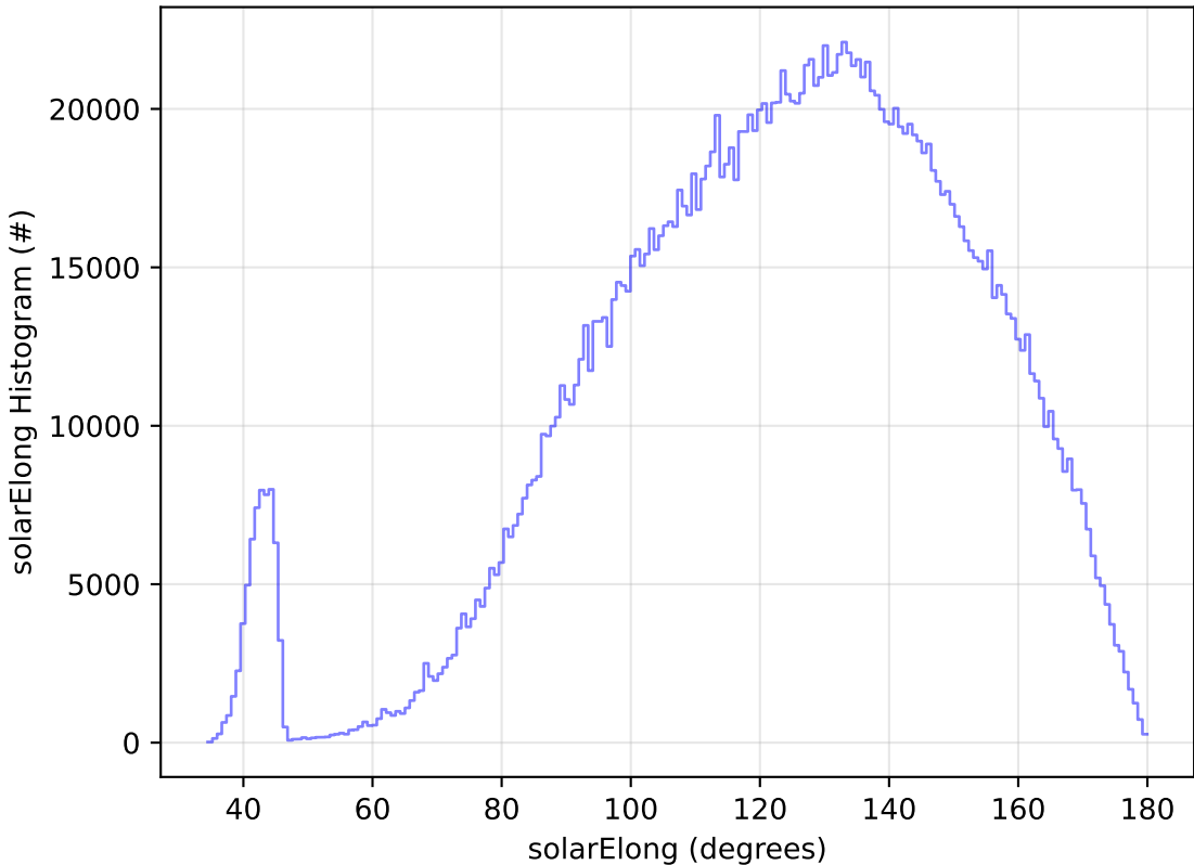
start_date_do-270v3.4_10yrs WFD all bands: solarElong Histogram
