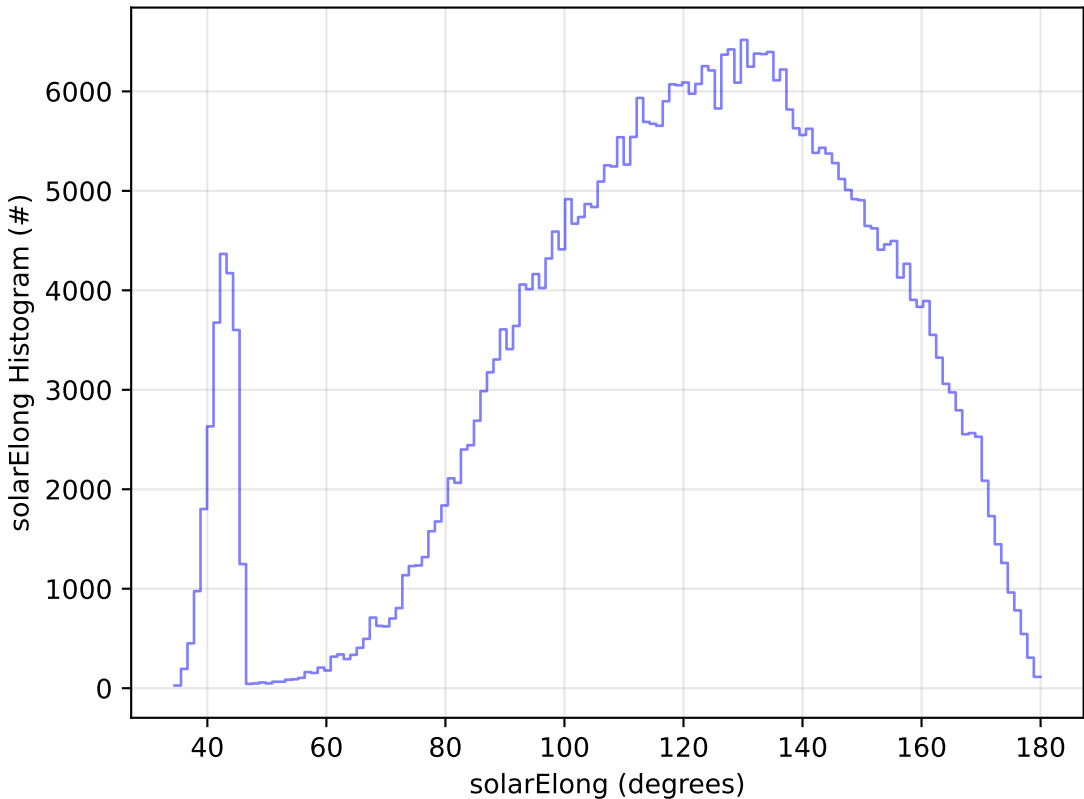
start_date_do-270v3.4_10yrs All sky z band: solarElong Histogram
