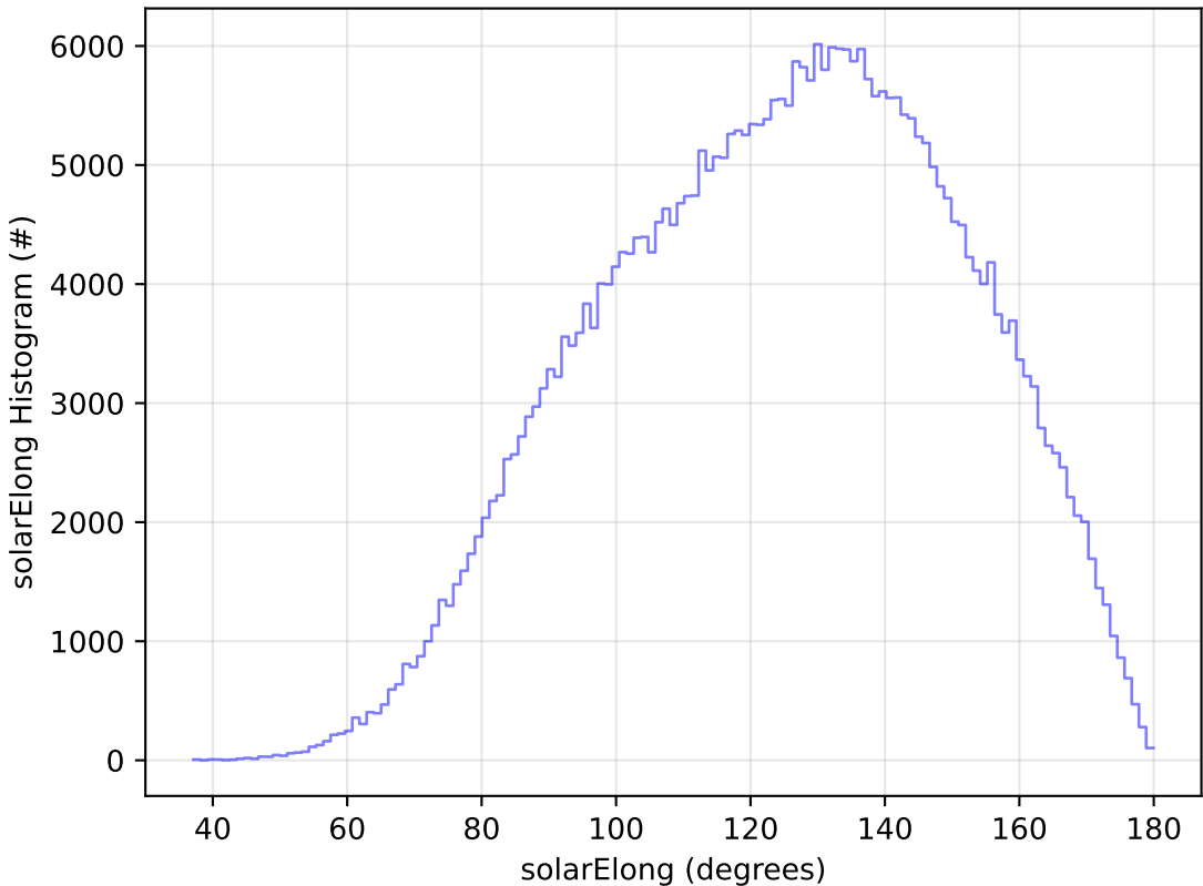
start_date_do-270v3.4_10yrs All sky y band: solarElong Histogram
