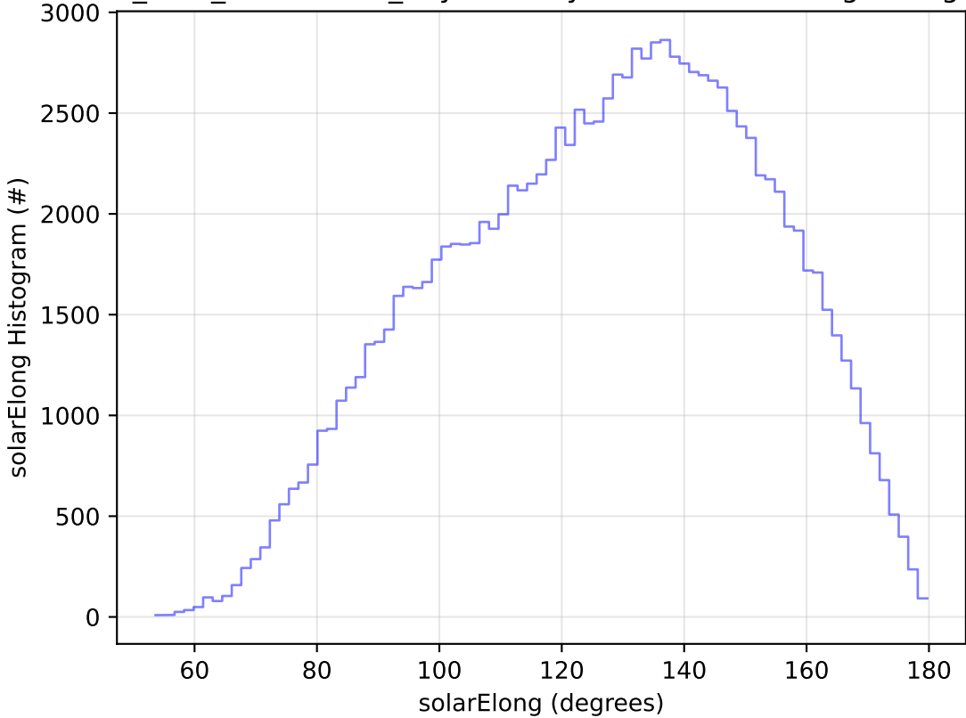
start_date_do-270v3.4_10yrs All sky u band: solarElong Histogram
