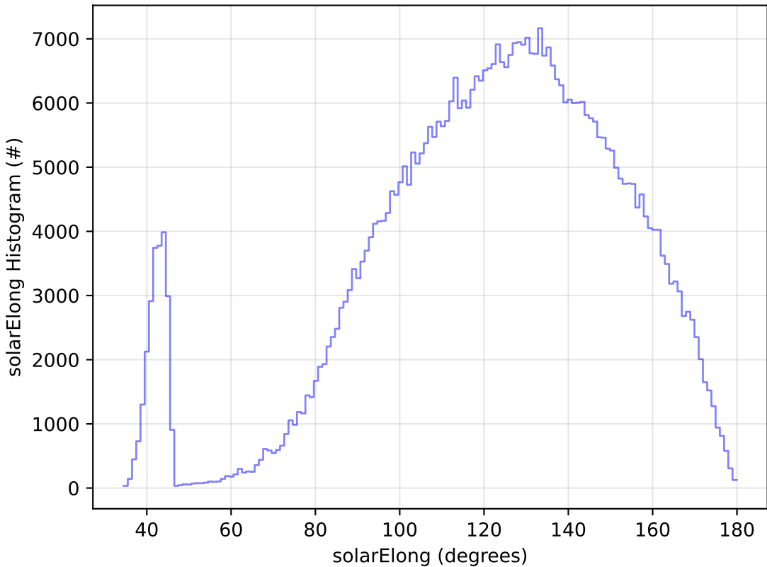
start_date_do-270v3.4_10yrs All sky i band: solarElong Histogram
