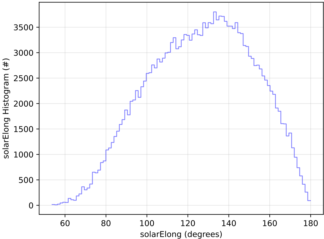
start_date_do-270v3.4_10yrs All sky g band: solarElong Histogram
