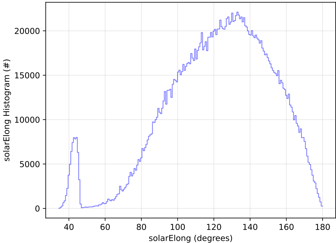
start_date_do-270v3.4_10yrs All sky all bands: solarElong Histogram
