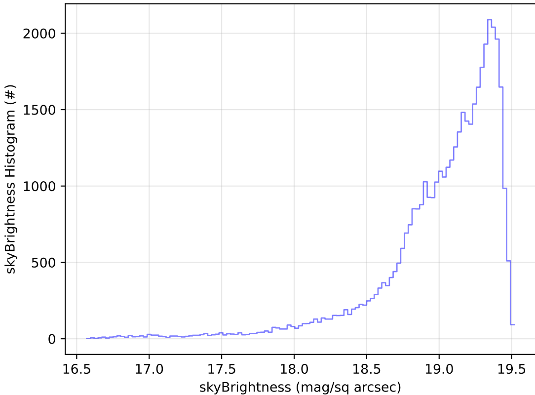
start_date_do-270v3.4_10yrs Yr 1 z band: skyBrightness Histogram
