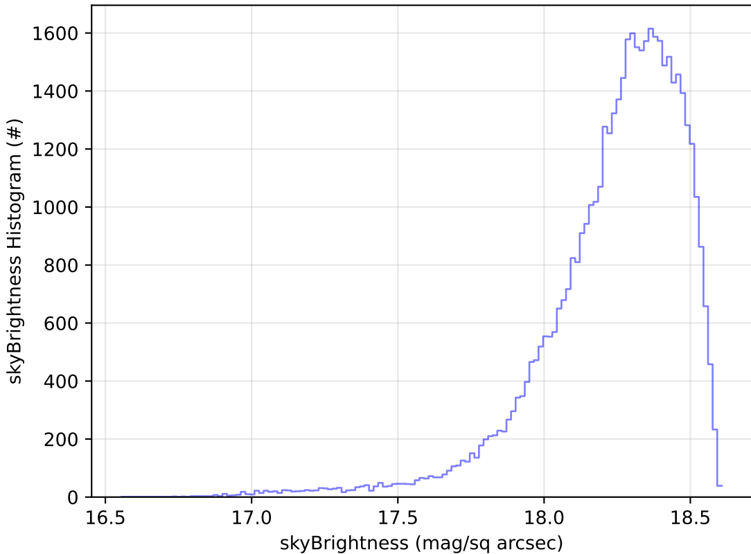
start_date_do-270v3.4_10yrs Yr 1 y band: skyBrightness Histogram
