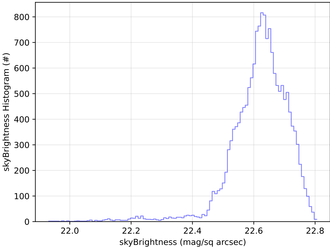
start_date_do-270v3.4_10yrs Yr 1 u band: skyBrightness Histogram
