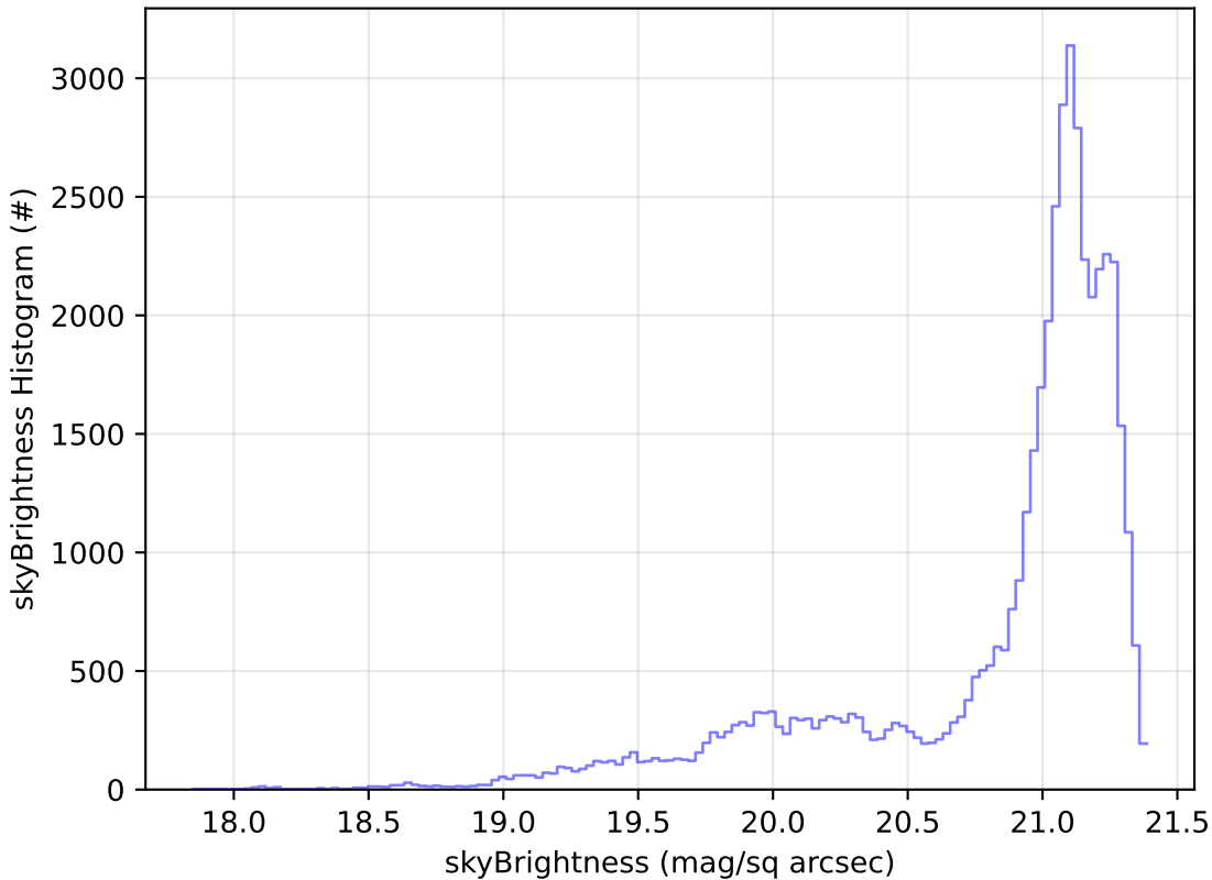
start_date_do-270v3.4_10yrs Yr 1 r band: skyBrightness Histogram
